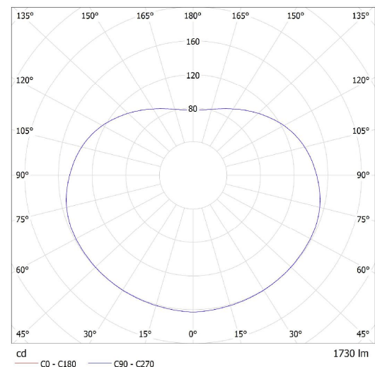
Lucis ZKS.L3.300.X POLARIS ZKS LED / LDC (Polar)
